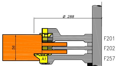
Raam-deurprofilering 40/56/68mm
