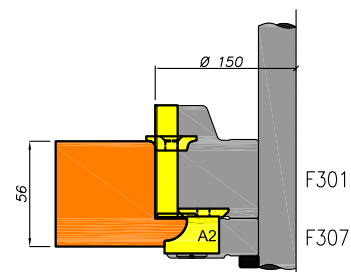
Raam-deurprofilering 40/56/68mm
