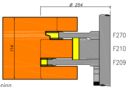
Raamprofilering
