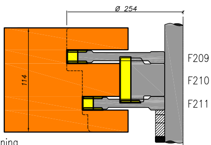
Raamprofilering
