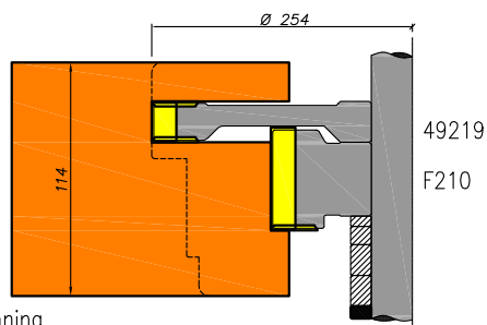
Raamprofilering
