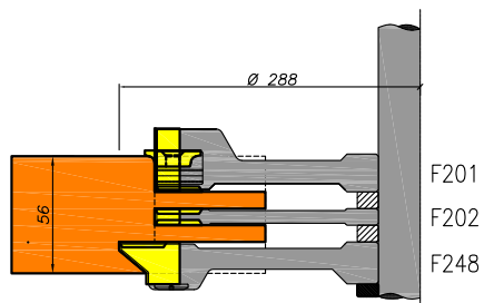
Raam-deurprofilering 40/56/68mm
