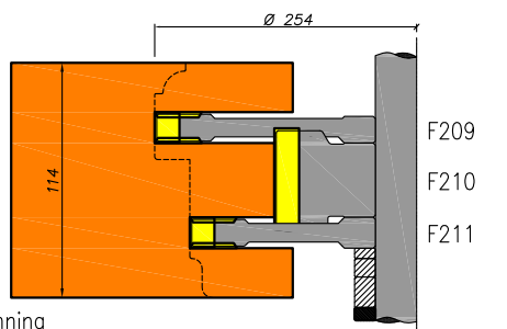
Raamprofilering
