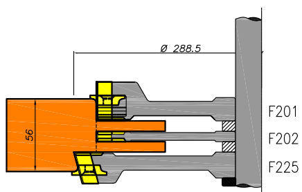
Raamprofilering
