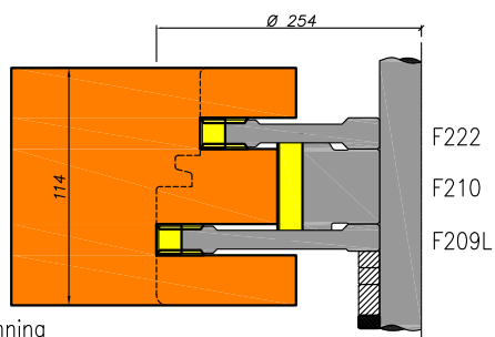
Raamprofilering
