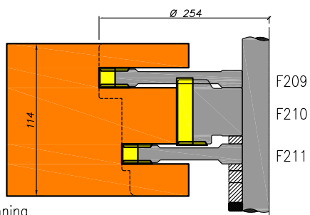
Raamprofilering
