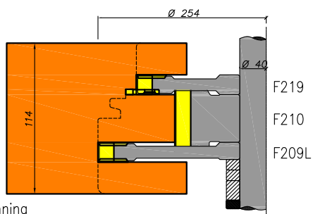
Raamprofilering
