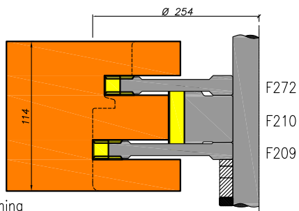
Raamprofilering
