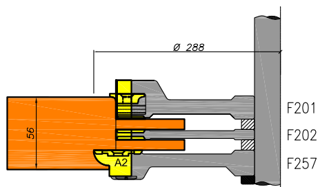
Raam-deurprofilering 40/56/68mm
