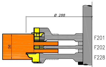
Raam-deurprofilering 40/56/68mm
