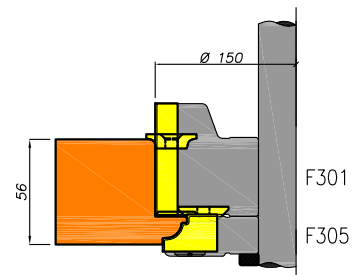
Raam-deurprofilering 40/56/68mm
